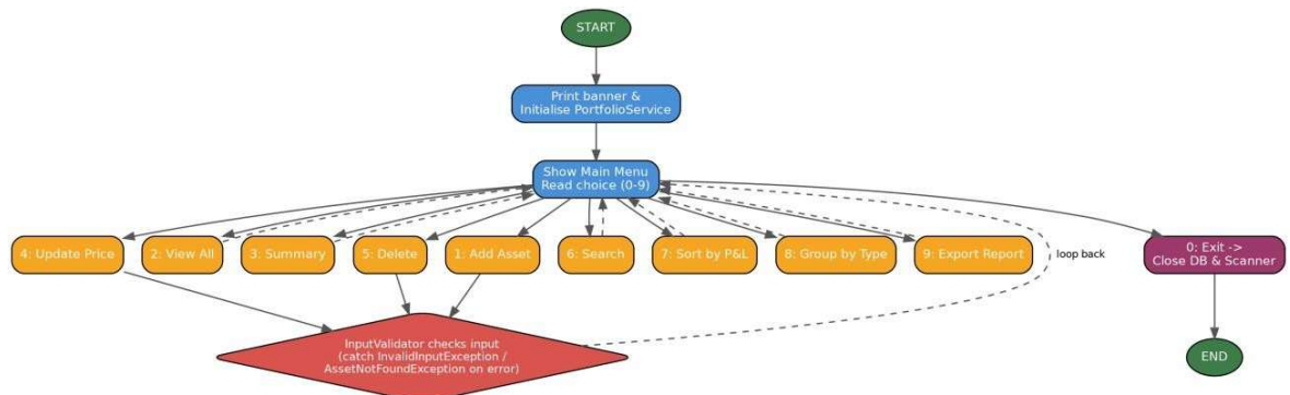
Figure 4. Workflow diagram — the main application loop in Main.main().
